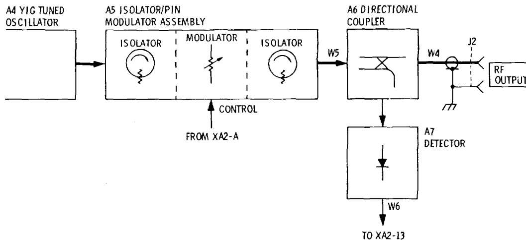
Figure 9-4. Partial Block Diagram (Option 001)
