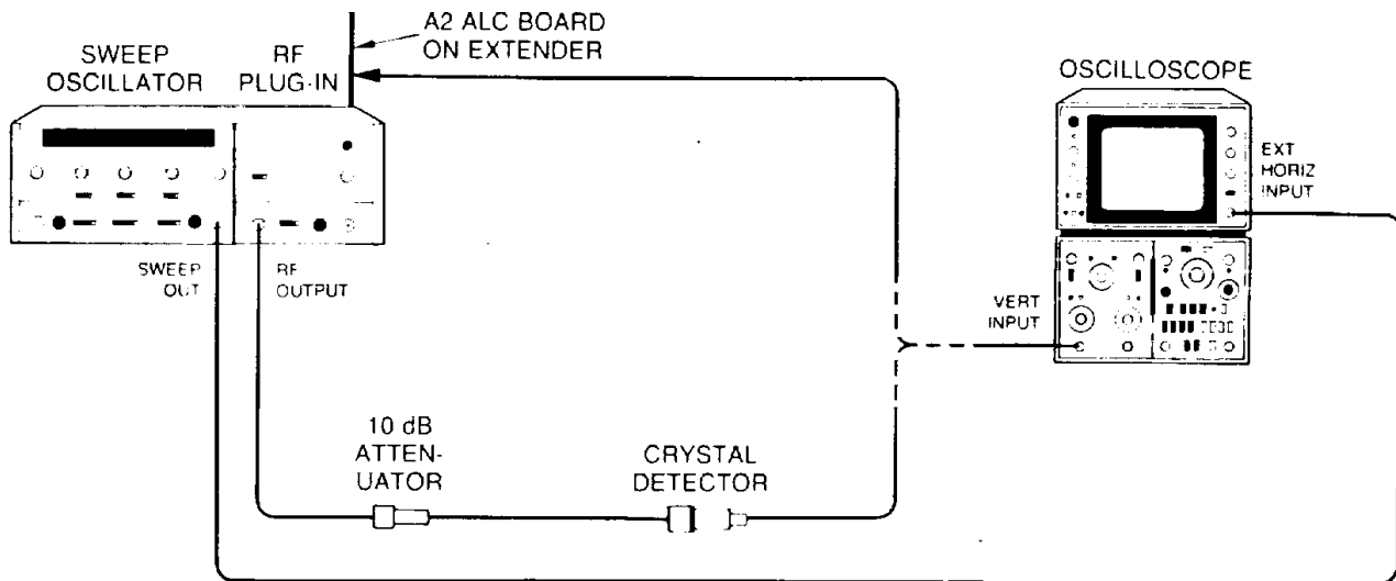
Figure 9-3. Internal Leveling Slope and Gain Adjustments Test Setup
