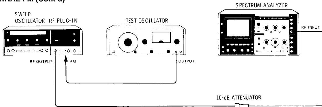
Figure 4-12. External Frequency Modulation Test Setup
