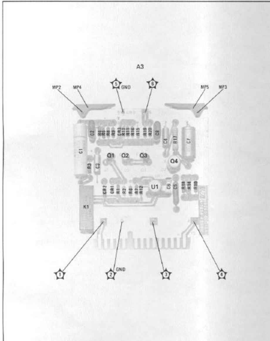
Figure 8-17. A3 FM Assembly, Components Location
